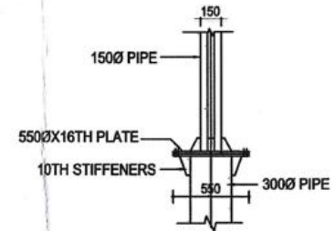
DETAIL A FOR PIPE JOINT
